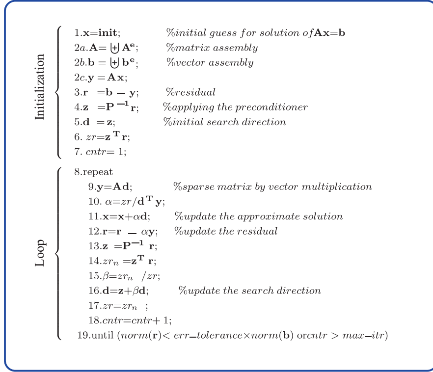
Figure 6.1: Pseudo-code for the conventional PCG method, \mathbf{x} = PCG(\mathbf{A}, \mathbf{b}) .
