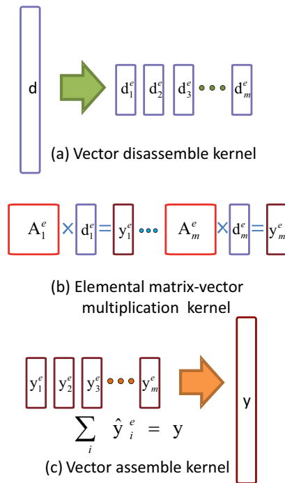
Figure 6.3: Schematic of kernels used to replace sparse matrix-vector multiplication in PCG algorithm with elemental matrix-vector multiplications.
