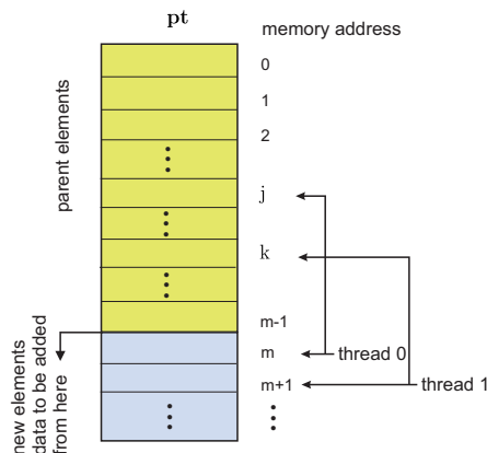
Figure 5.9: Updating nodal-elemental matrix \mathbf{pt} for bisected elements to include mesh data of newly added elements.
