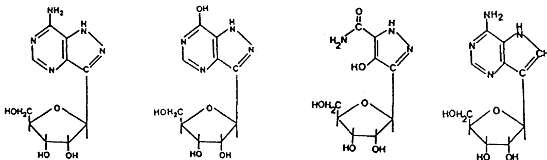
Formycin A
